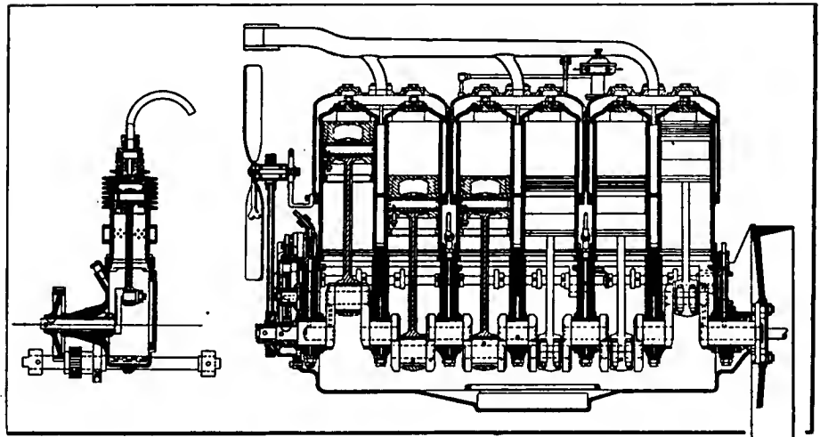
Fig. 8—Lateral cross-section of a Pierce-Arrow motor with seven-bearing crankshaft and the section of the air pump for tire inflation
